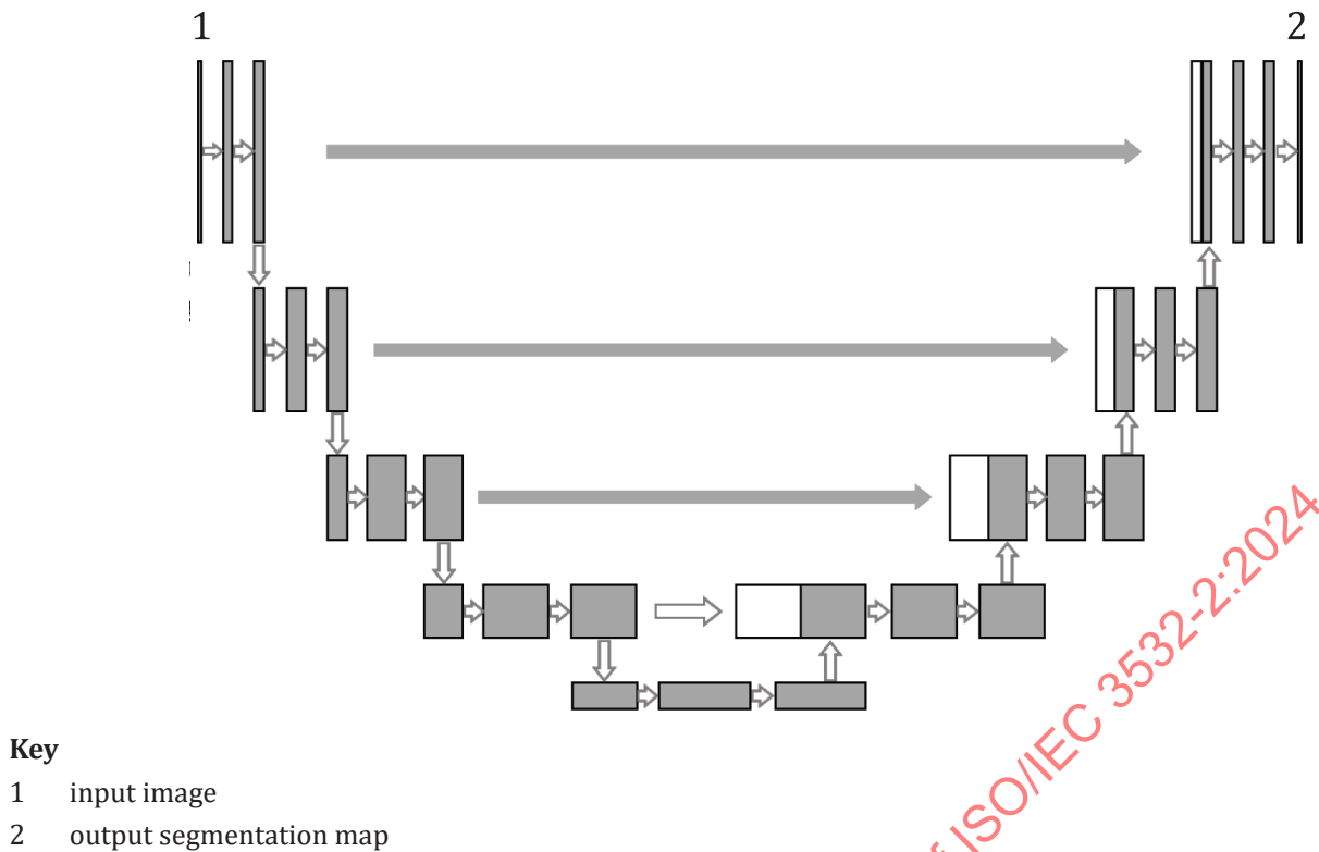
Figure D.2 — U-Net structure
