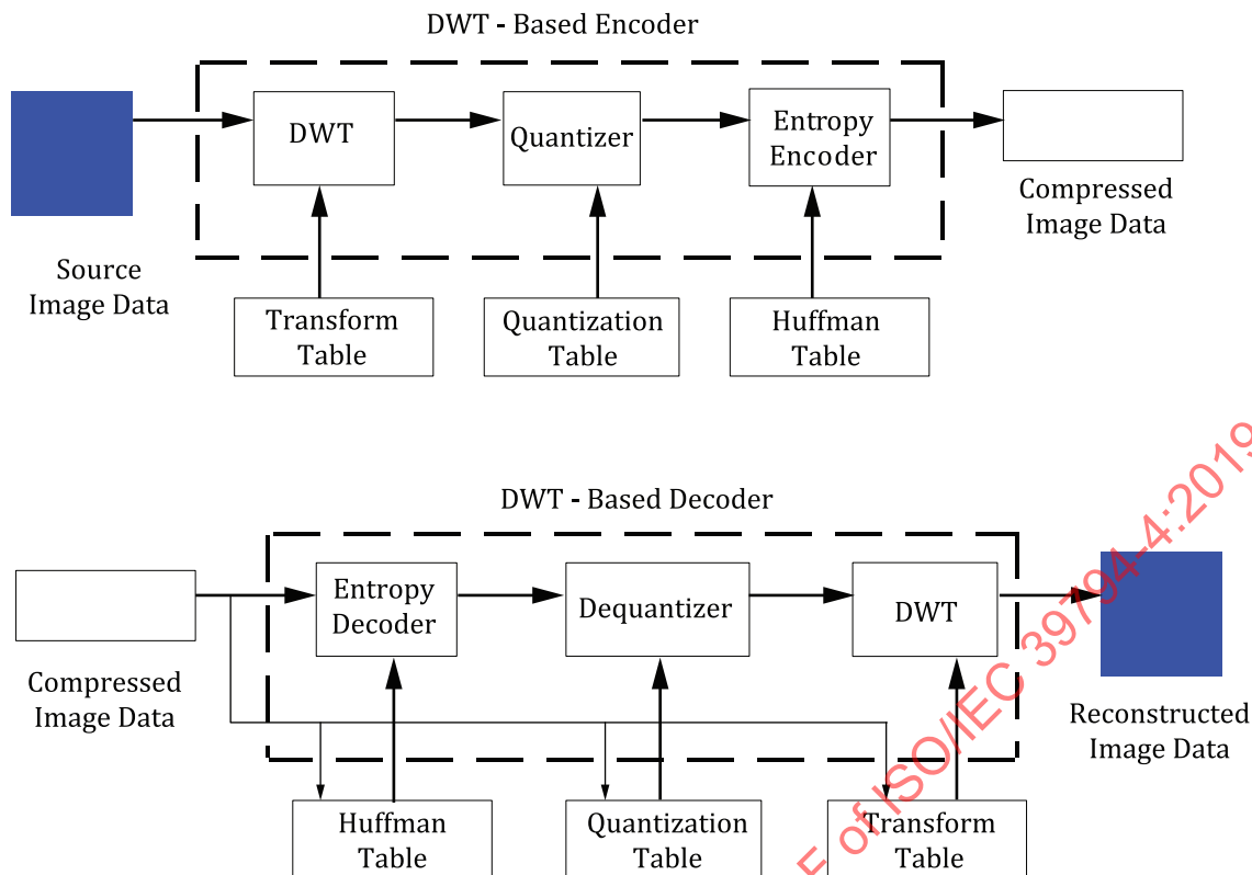
Figure F.1 — DWT-based encoder and decoder simplified diagram
