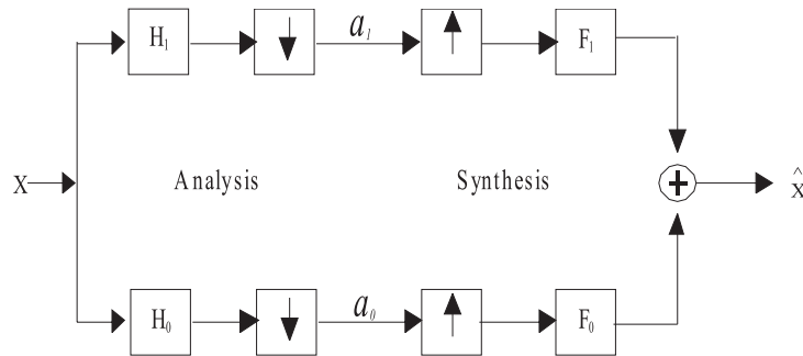
Figure F.2 — Two-channel subband coder
