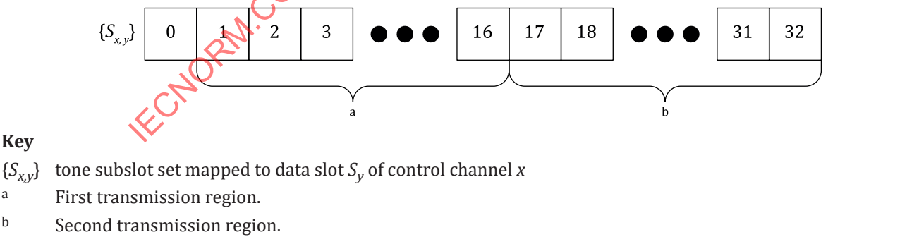
Figure 17 — Transmission region of collision tone in TSBtype0
