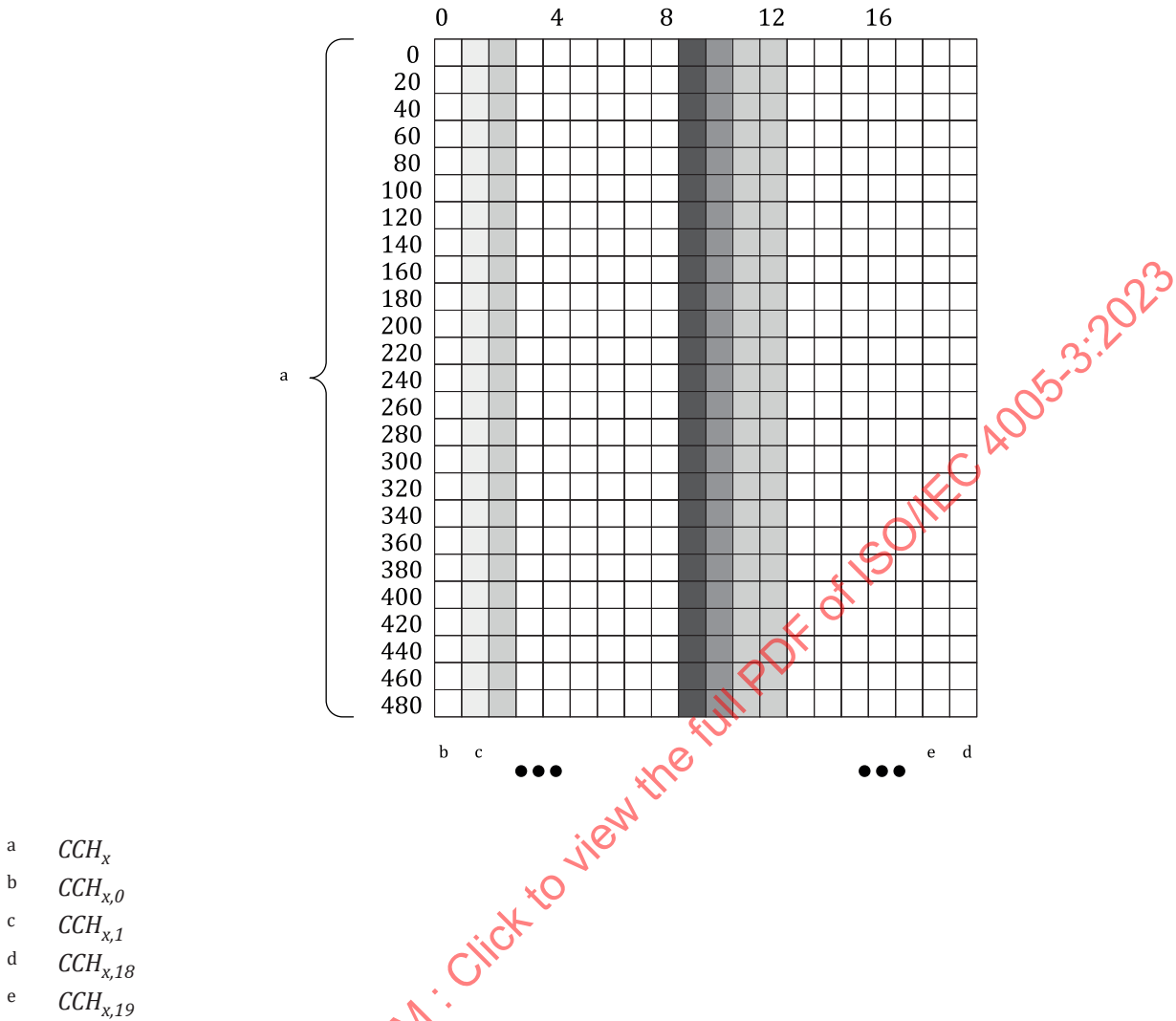
Figure 4 — Subchannel structure of control communication in even frame
