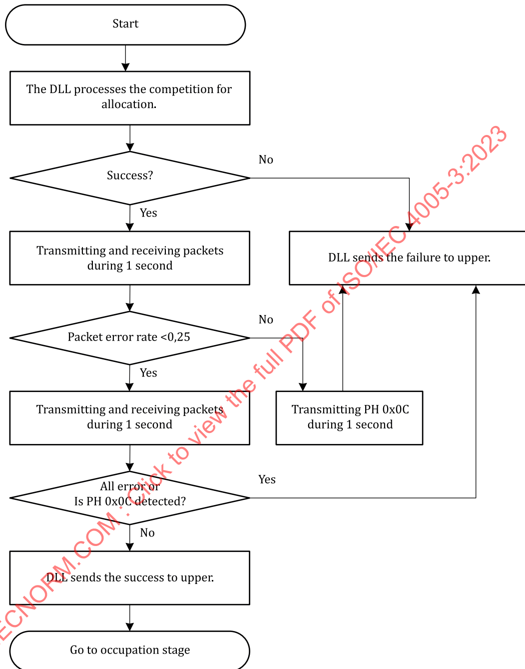
Figure 16 — Resource allocation competition and generated link confirmation
