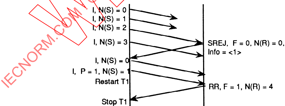
Figure C.1 — I frame recovery due to SREJ frame with F bit set to "0"
