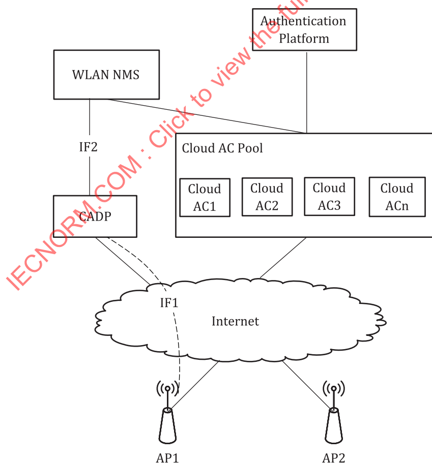
Figure 1 — CADP-based WLAN architecture
