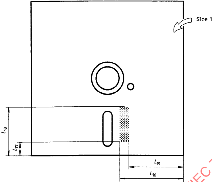
Figure 6 — Pressure pad area
