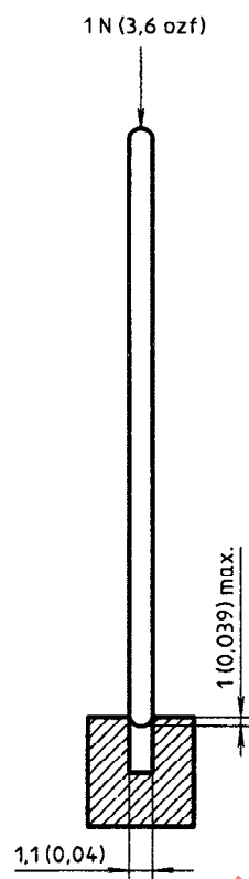
Figure A.2 — Measuring gauge for minimum thickness
