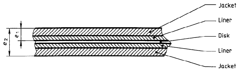
Figure 4 — Cartridge thickness
