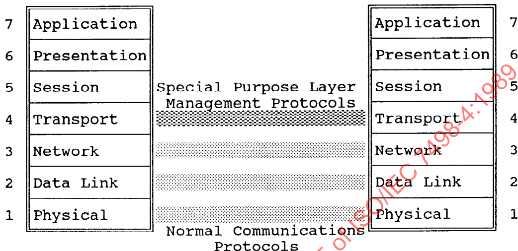
Figure A.2 - (N)-Layer Management Exchange
