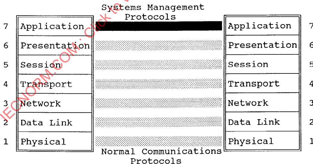
Figure A.1 - Systems Management Information Exchange
