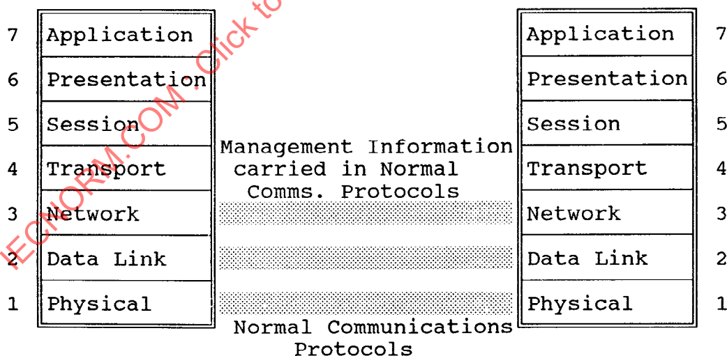
Figure A.3 - (N)-Layer Operation
