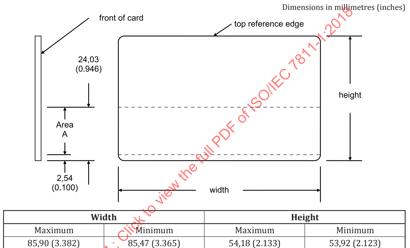
Figure 1 — Embossed card dimensions
