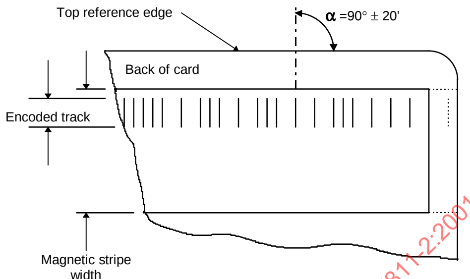
Figure 9 — Angle of recording
