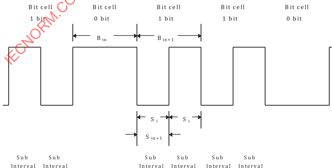
Figure 11 — Flux transition spacing variation
