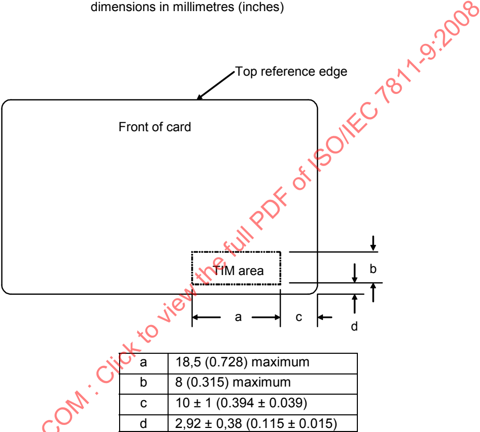
Figure 1 — Recommended TIM area
