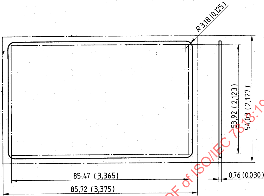
Figure 1 — Card dimensions
