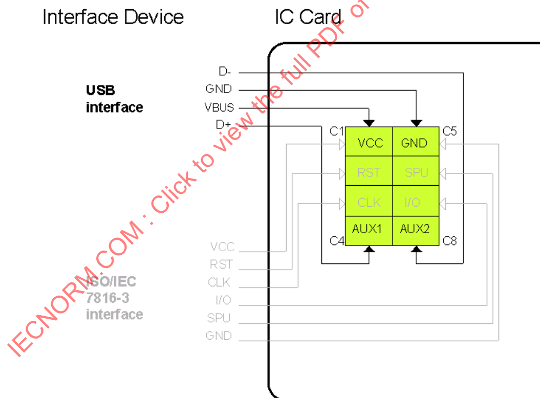
Figure 1 — Assignment of contacts for a USB integrated circuit card
