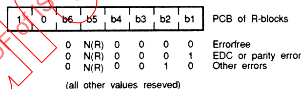
Figure 14 - Coding of R-block PCB
