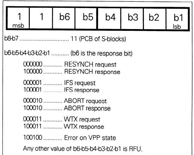
Figure 19 — Coding of S-block PCB
