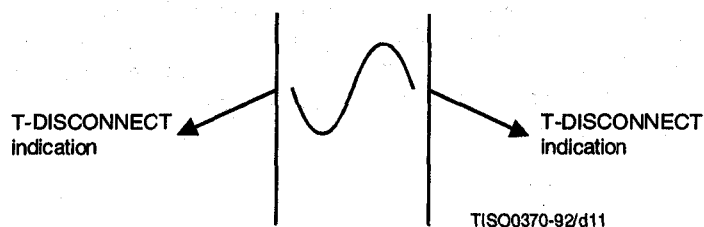
Figure 10 – Sequence of primitives in a TS provider invoked release
