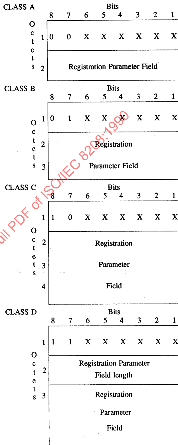
Figure 30 — Generalized Formats of Registration Elements
