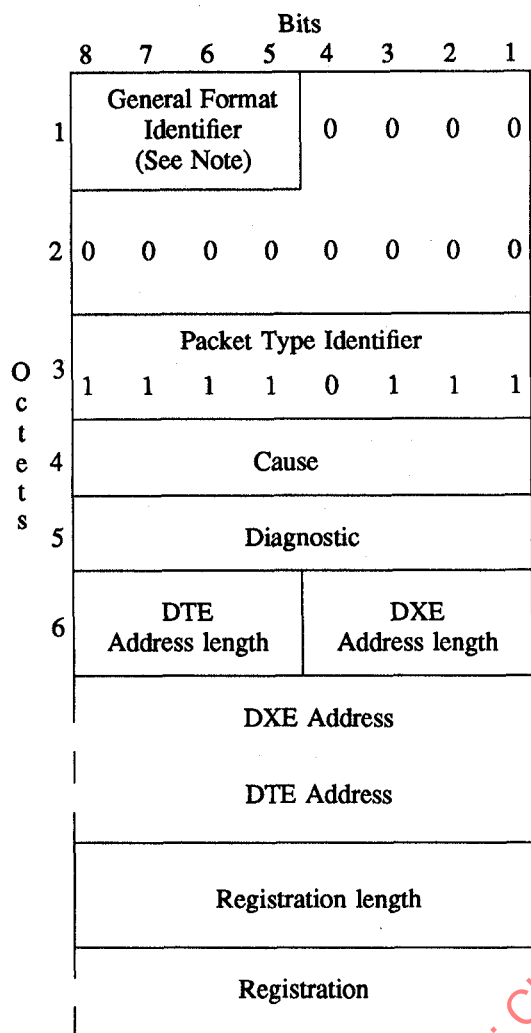
NOTE — Coded 0001 (modulo 8) or 0010 (modulo 128) Figure 27 — REGISTRATION CONFIRMATION Packet Format
