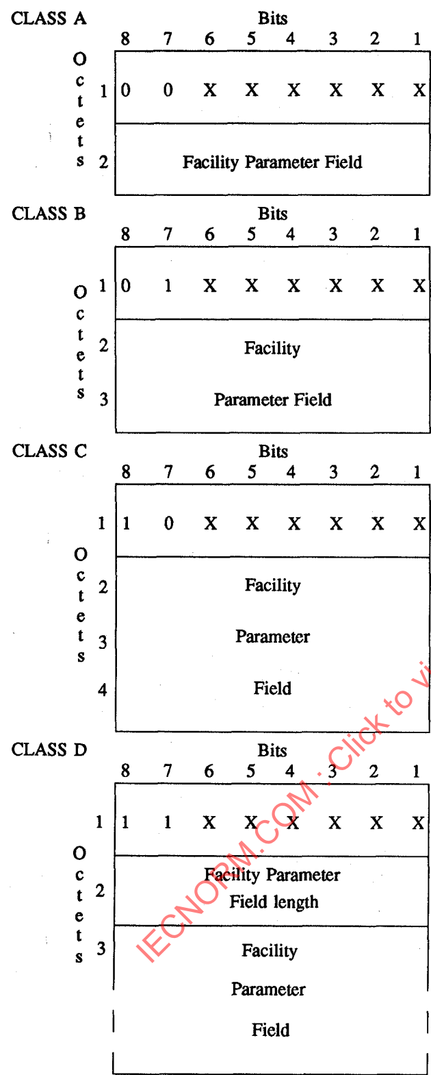
Figure 29 — Generalized Formats of Facility Elements
