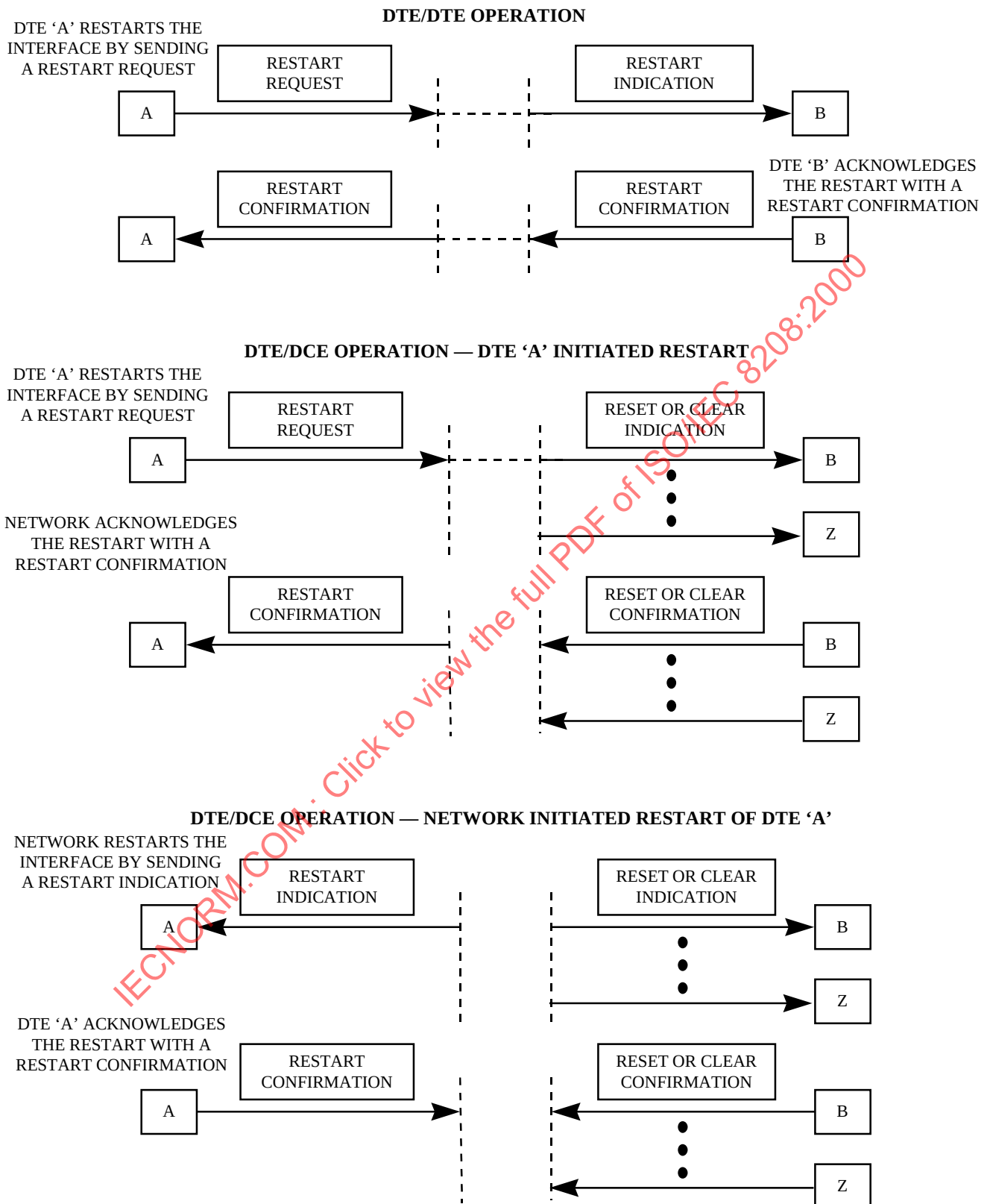
Figure 3 — Restart Schematic
