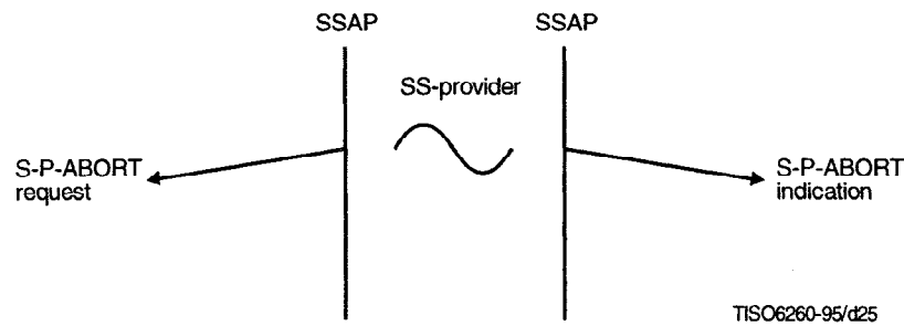
Figure 24 – P-abort time sequence diagram
