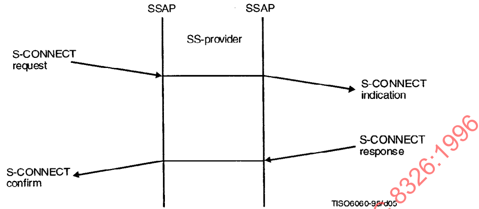
Figure 4 – Scssion connection establishment time sequence diagram
