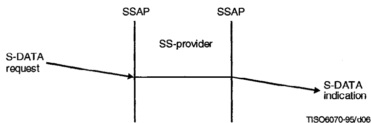
Figure 5 – Normal data transfer time sequence diagram
