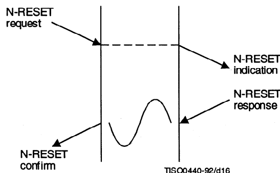
Figure 15 – Sequence of primitives in NS user invoked reset
