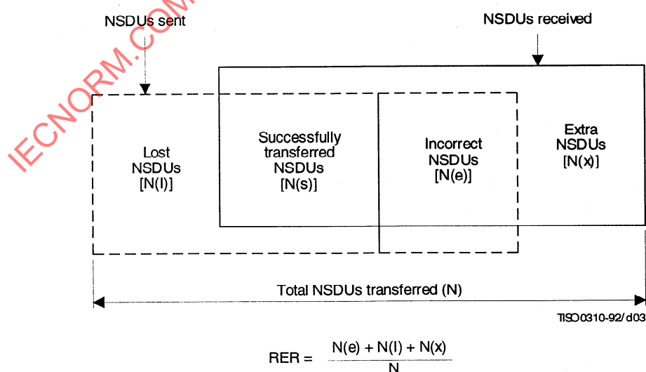
Figure 2 – Components of residual error rate
