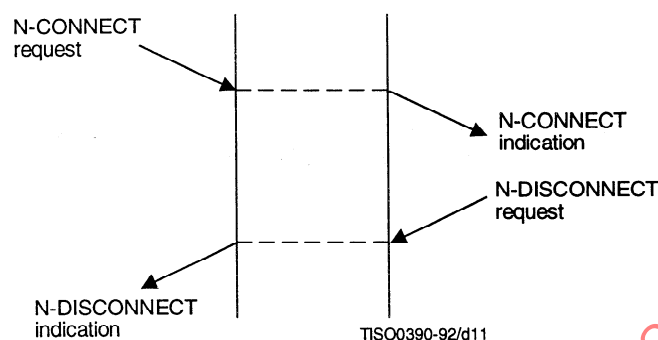
Figure 10 – Sequence of primitives in NS user rejection of an NC establishment attempt
