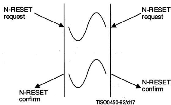
Figure 16 – Sequence of primitives in simultaneous NS user invoked reset
