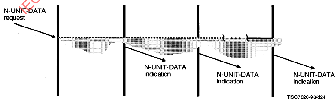
Figure 21b – Sequence of primitives in a multicast network-connectionless-mode transmission
