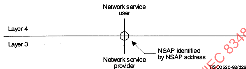
Figure A.2 – NSAP address
