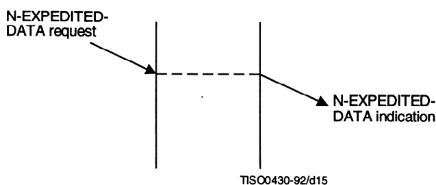
Figure 14 – Sequence of primitives in expedited data transfer
