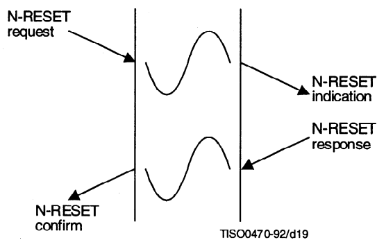
Figure 18 – Sequence of primitives in simultaneous NS user and NS provider invoked reset
