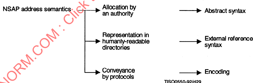
Figure A.5 – Relationship of NSAP address semantics and syntax
