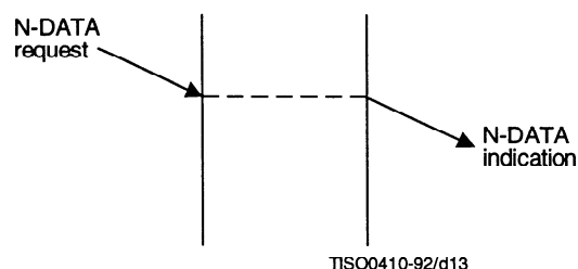
Figure 12 – Sequence of primitives in data transfer
