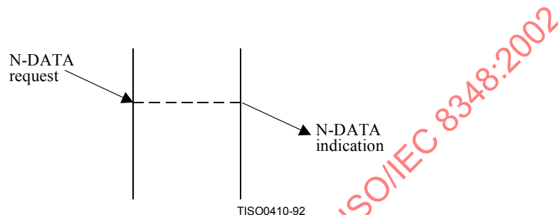
Figure 12 – Sequence of primitives in data transfer
