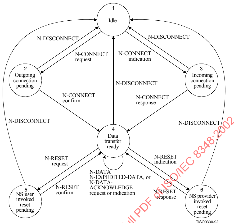
Figure 4 – State transition diagram for sequences of primitives at an NC end-point
