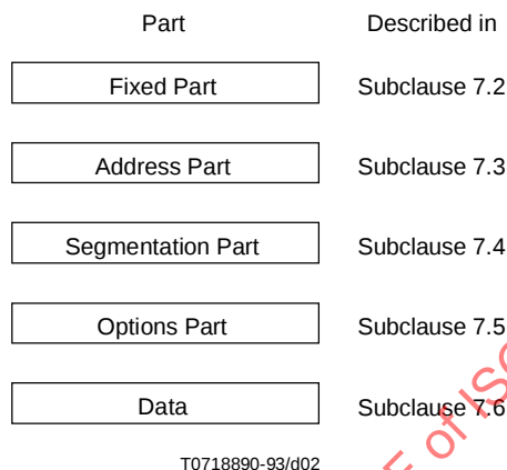
Figure 1 – PDU structure
