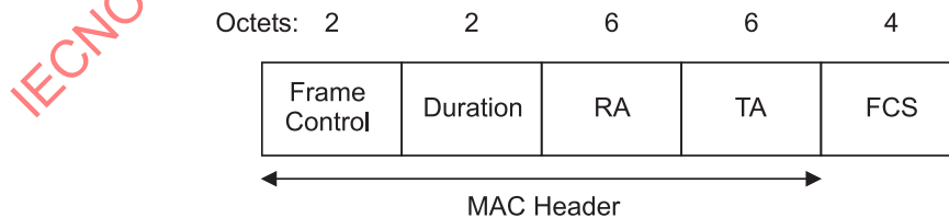
Figure 16—RTS frame
