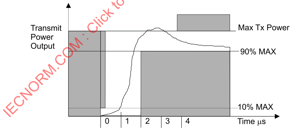
Figure 97—Transmit power-on ramp
