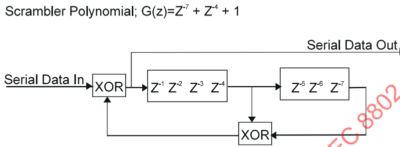
Figure 89—Data scrambler
