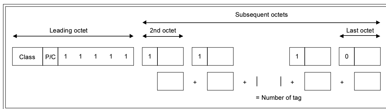
Figure 4 – Identifier octets (high tag number)
