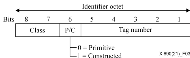
Figure 3 – Identifier octet (low tag number)
