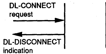
Figure 12 - Sequence of primitive in DLS Provider rejection of a DLC establishment attempt
