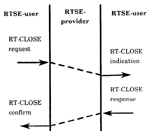
Figure 3 - RT-CLOSE service-primitives
