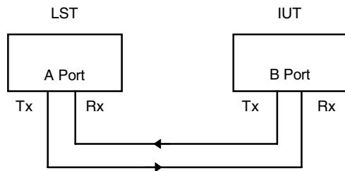
Figure 3 - Tester Configuration for Indicated Cases
