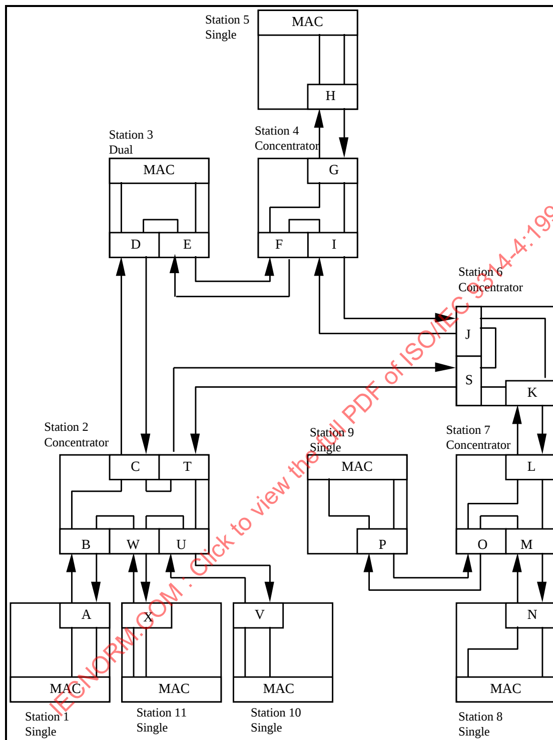
Figure 2 – FDDI Topology Example
