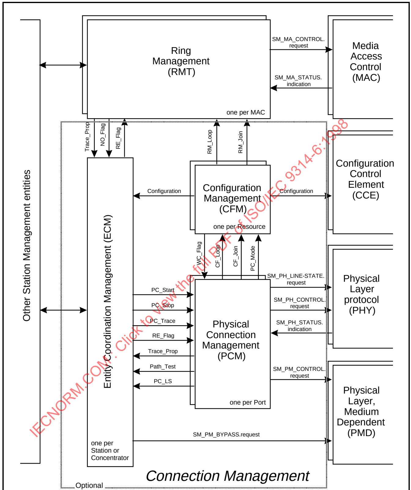
Figure 9 – Connection Management structure
