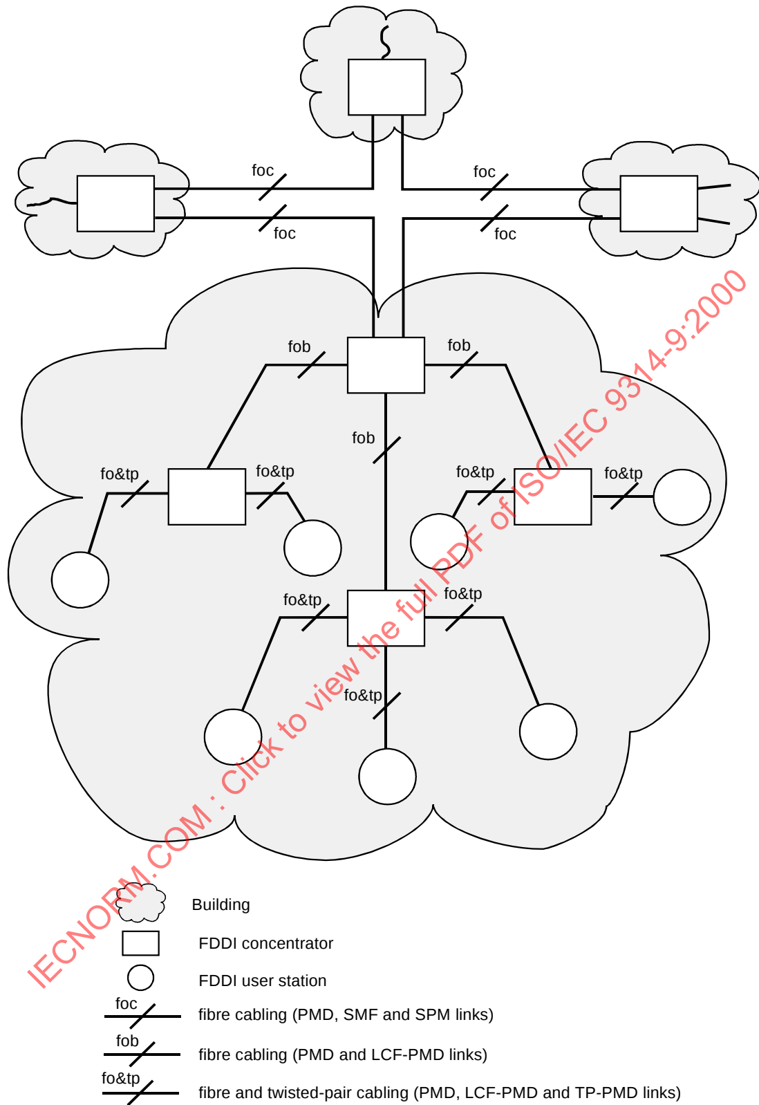
Figure 3 — FDDI representative distribution environment example
