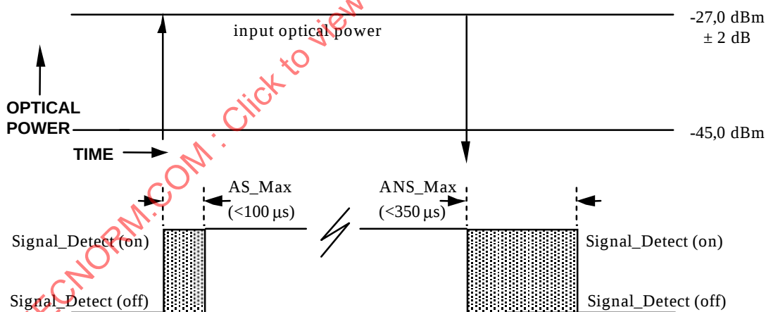
Figure 5 — Signal detect thresholds and timing
