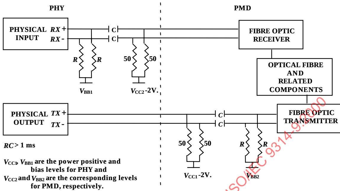
Figure C.2 – Test configuration for a.c. coupled components
