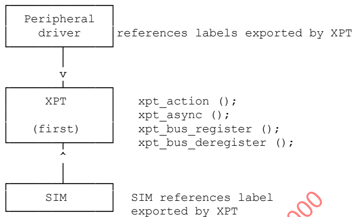
Figure 2 – CAM layers
