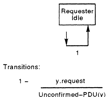
Figure 4 - Unconfirmed Service as seen by the Service Requester
