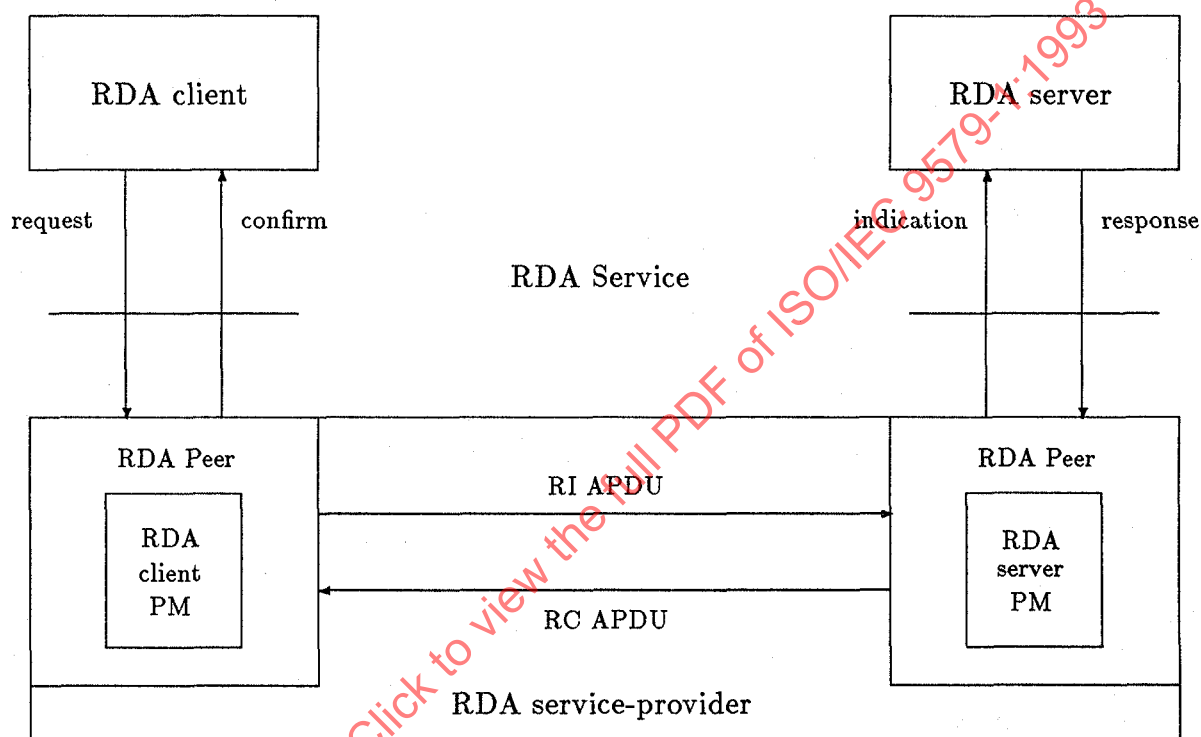
Figure 4 – Relationship of RDAPM to RDA model
