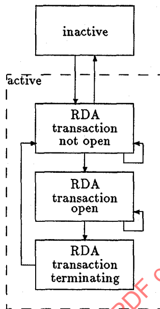
Figure 2 – Overview of RDA states
