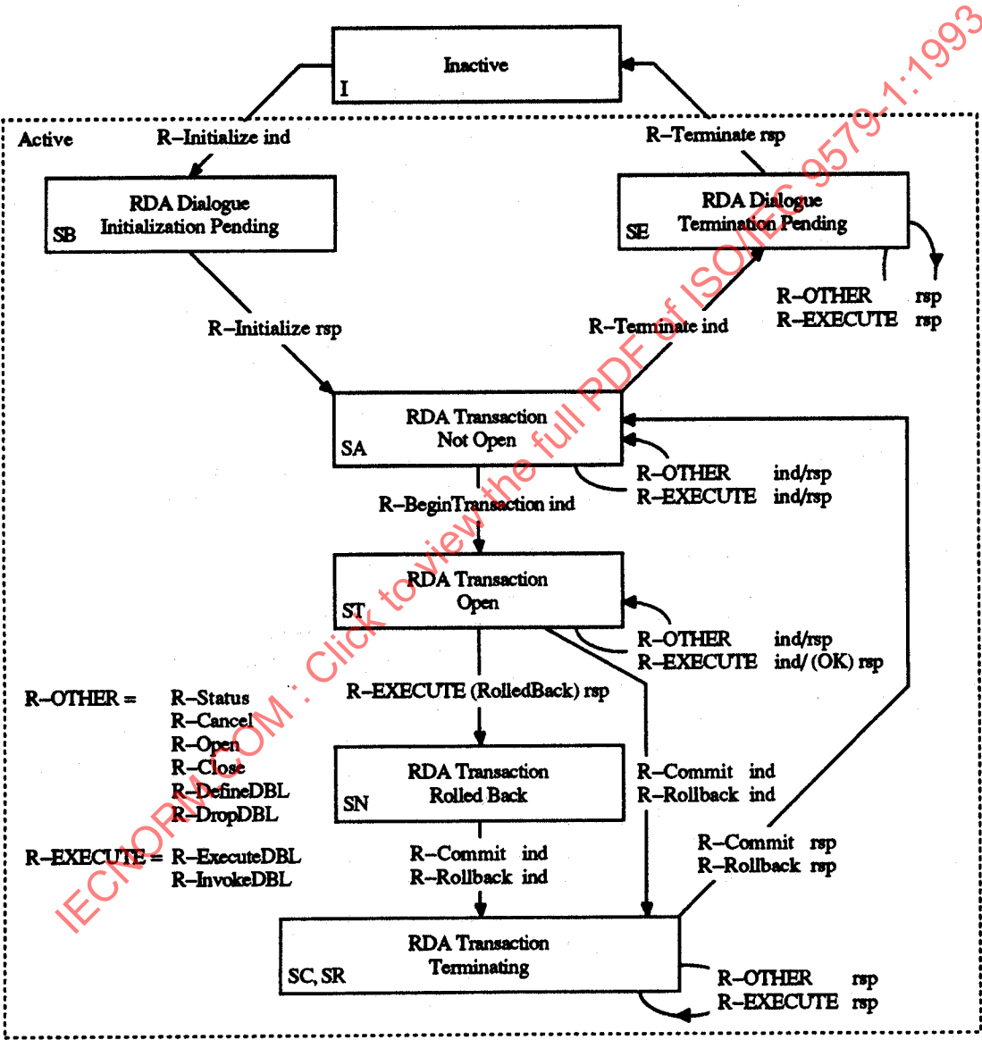
Figure 6 – State transition diagram for RDA Basic application-context – RDA server
