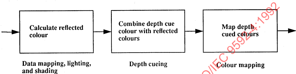
Figure 10 — The conceptual rendering pipeline
