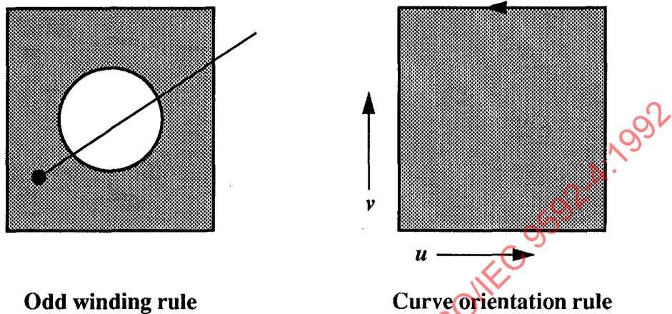
Figure 5 — Parameter space mapping rules for trimming curves (The mapped region is shaded)
