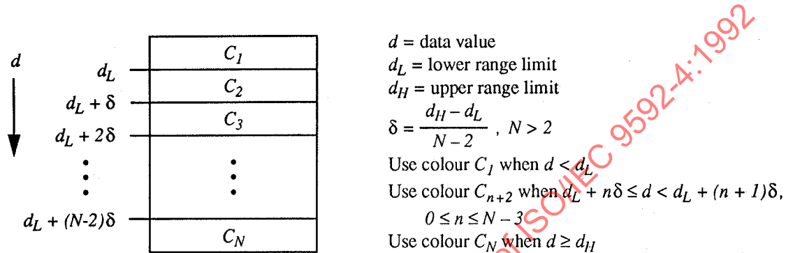
Figure 11 — UNIFORM data mapping of data values to colours
