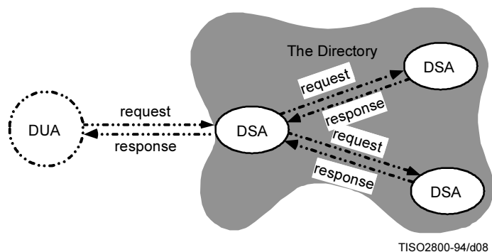
Figure 7 – Multi-chaining
