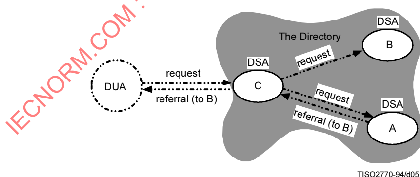
Figure 5a – Referrals
