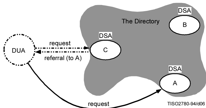
Figure 5b – Referrals
