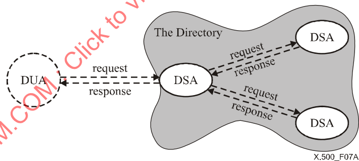
Figure 7a – Multi-chaining
