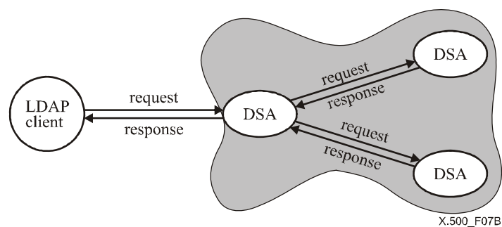
Figure 7b – Multi-chaining
