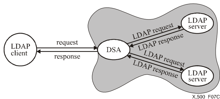
Figure 7c – Multi-chaining
