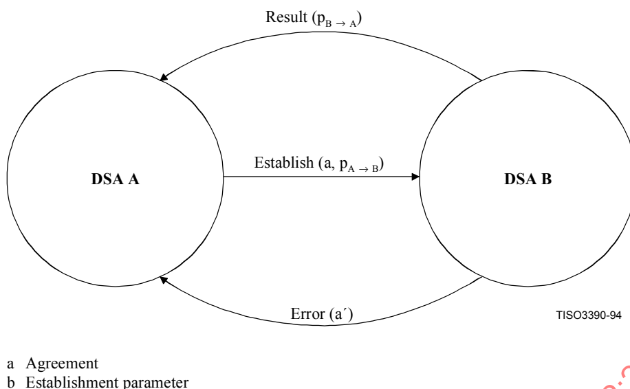
Figure 26 – DSA with Role B initiating establishment
