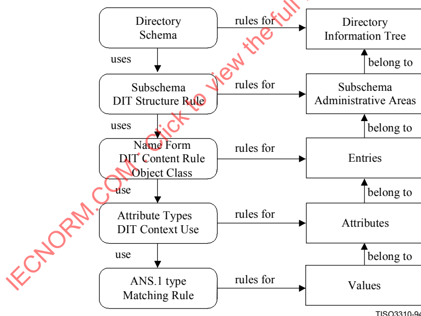
Figure 11 – Overview of Directory Schema
