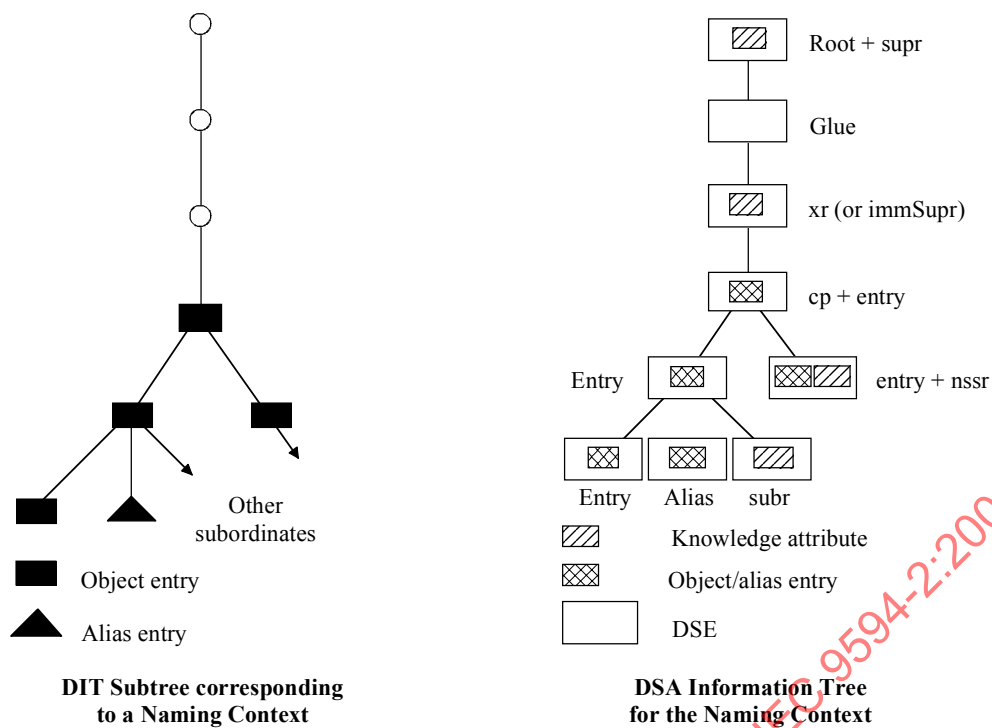
Figure 22 – DSEs for a Naming Context
