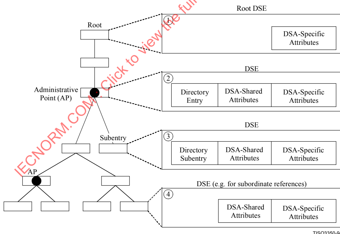
Figure 21 – A DSA Information Tree
