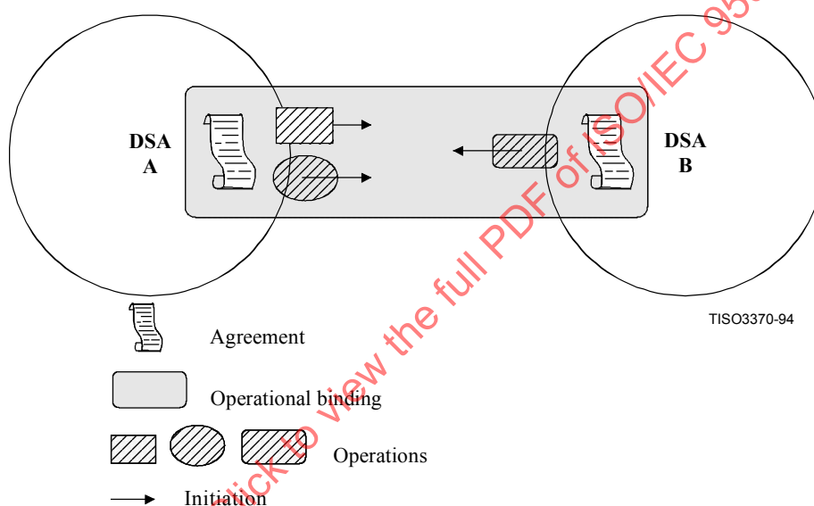
Figure 23 – An operational binding
