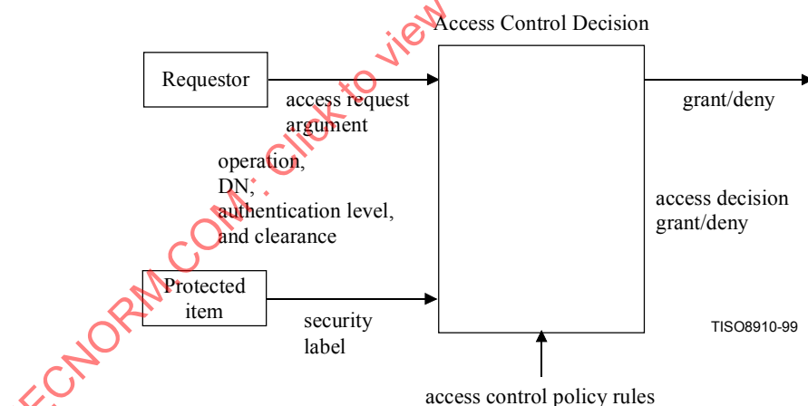
Figure 18 – Rule-based Access Control Decision Model
