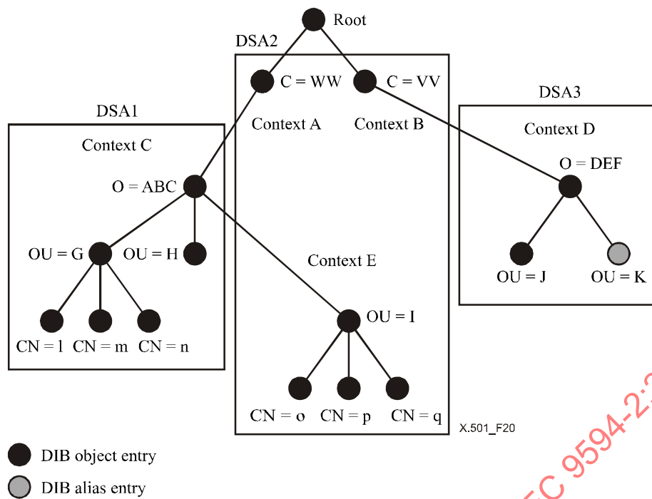
Figure 20 – Hypothetical DIT
