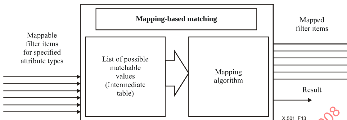
Figure 13 – Mapping-based matching
