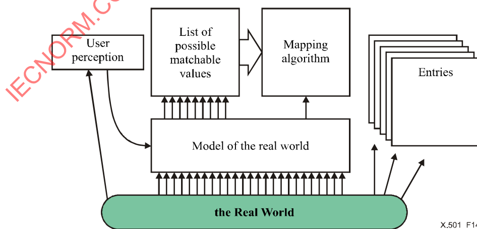
Figure 14 – Information derivation
