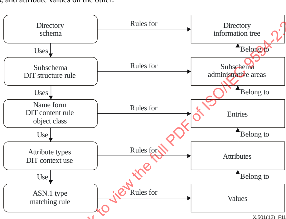
Figure 11 – Overview of Directory Schema
