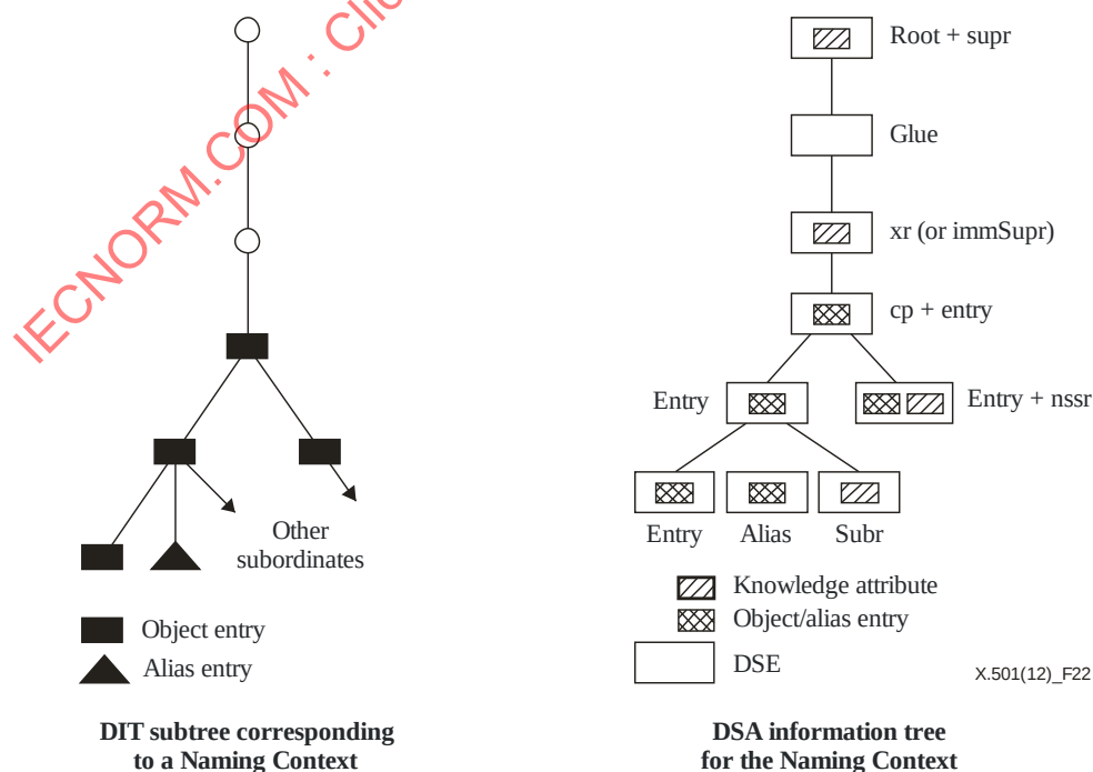
Figure 22 – DSEs for a Naming Context
