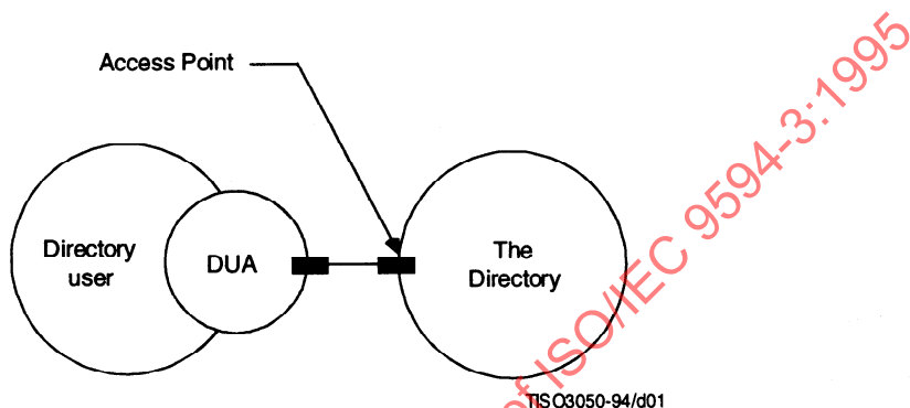
Figure 1 – Access to the Directory
