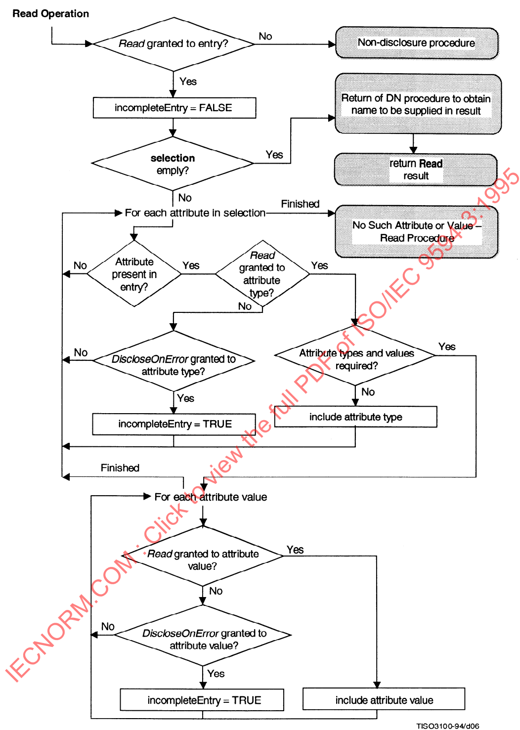
Figure B.5 – Read Operation
