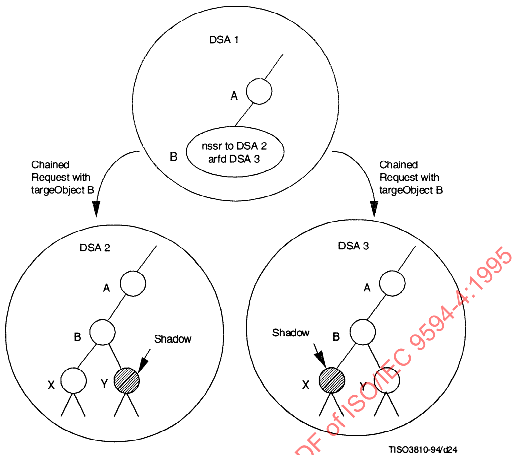
Figure 22 – Multi-chaining caused by NSSR during Name Resolution
