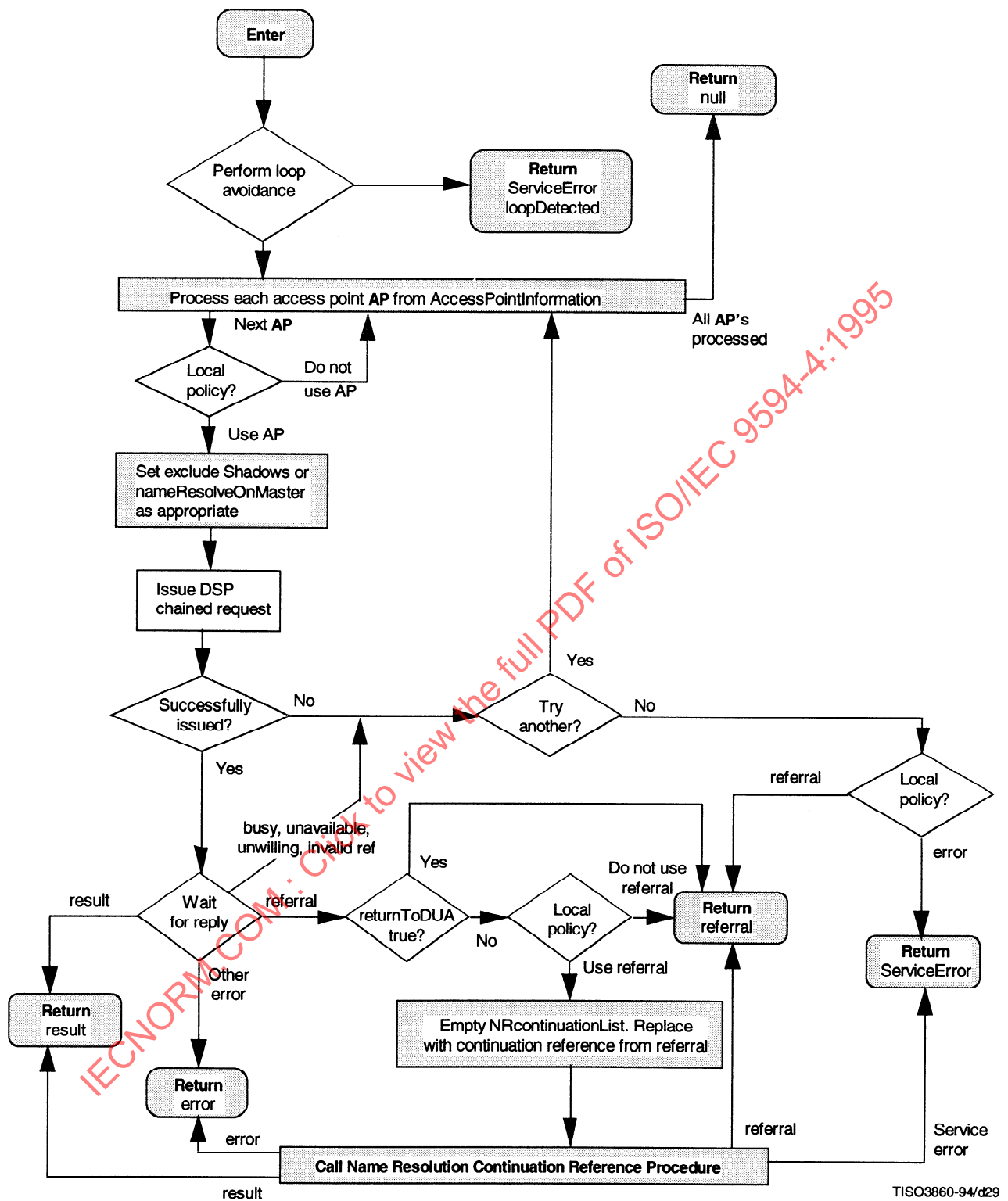
Figure 27 – APInfo procedure
