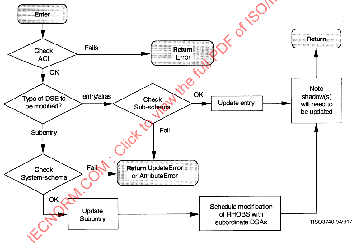
Figure 15 – Modify Entry procedure
