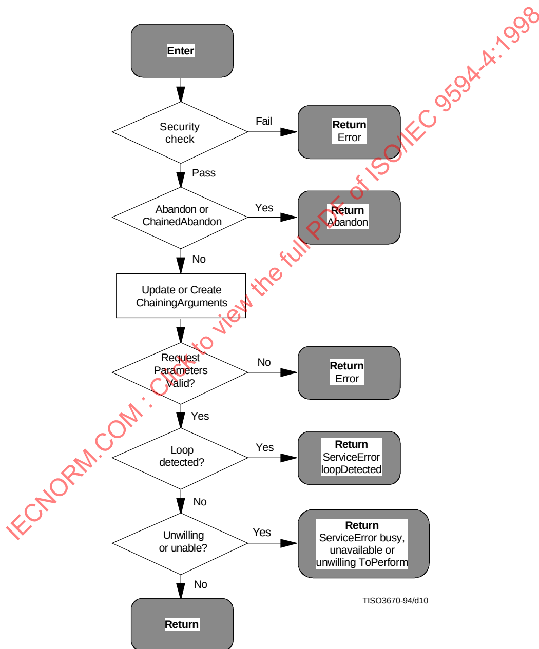
Figure 8 – Request Validation procedure
