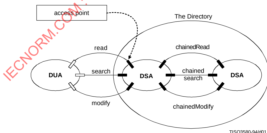
Figure 1 – Objects of the distributed Directory model
