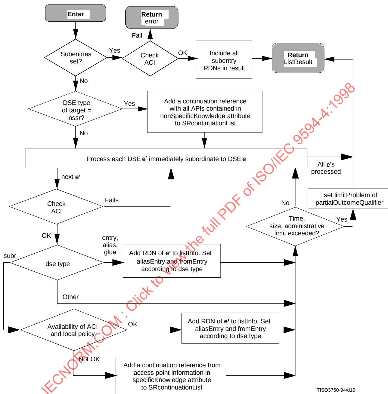
Figure 17 – List (I) procedure
