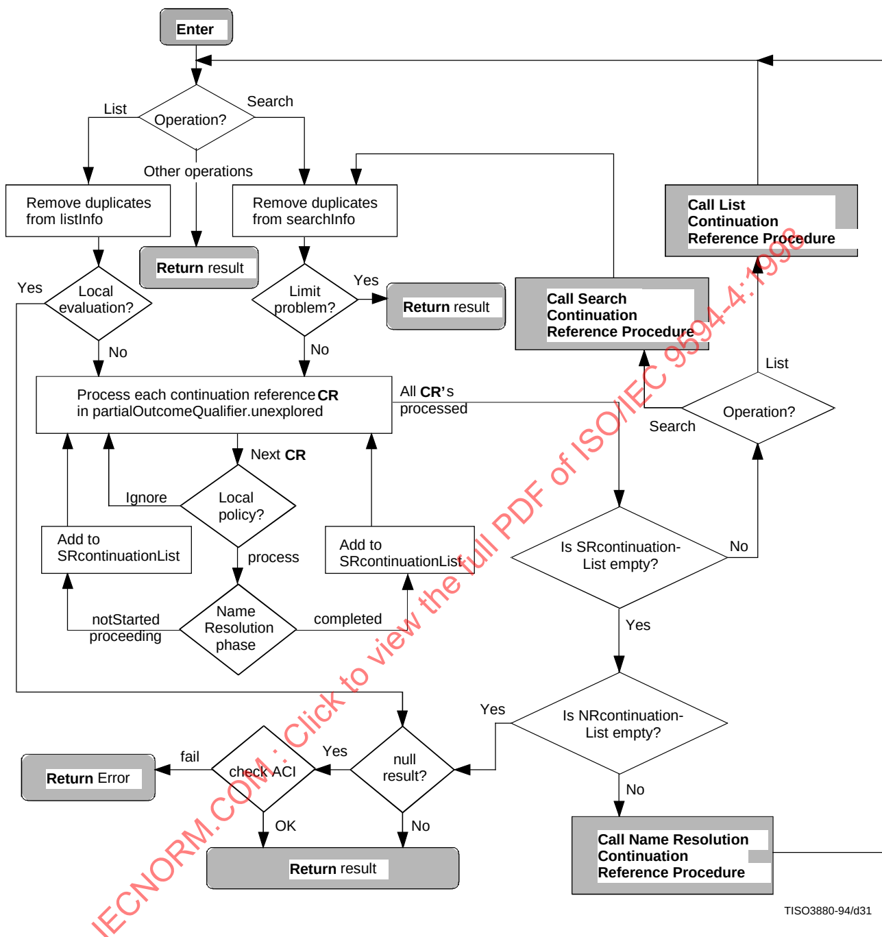
Figure 29 – Results Merging procedure
