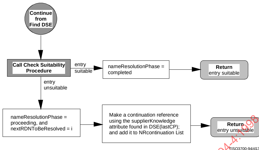
Figure 11 – Target Found sub-procedure
