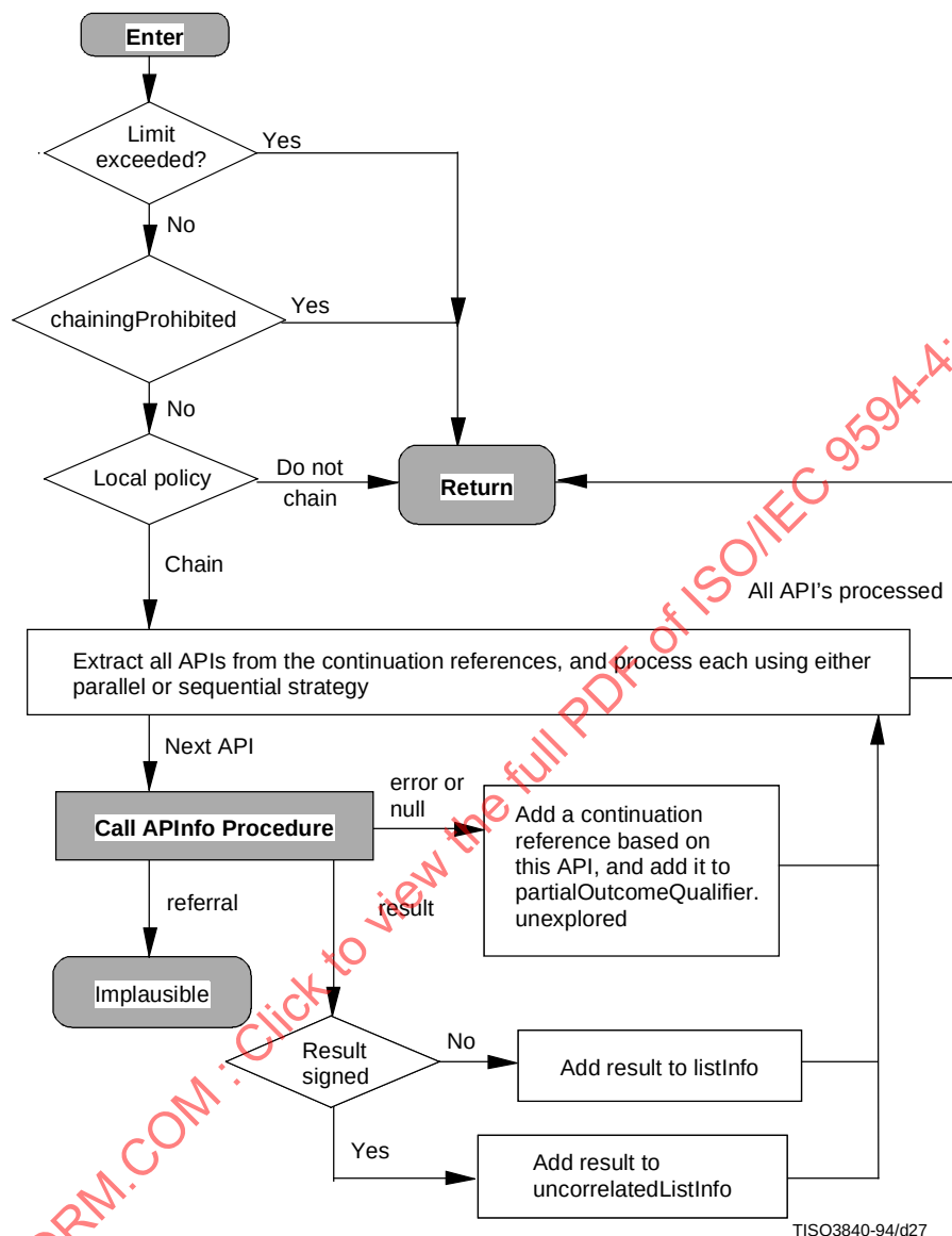
Figure 25 – List Continuation Reference procedure
