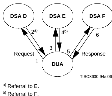
Figure 4b – Referral mode (DUA acts on referrals)
