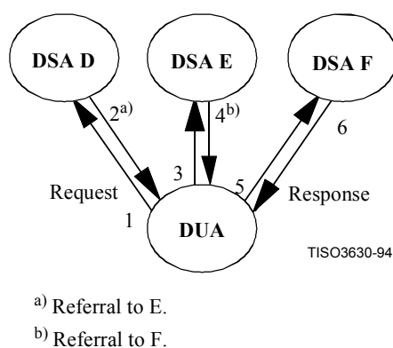
Figure 4b – Referral mode (DUA acts on referrals)
