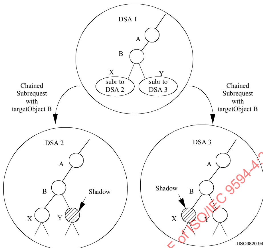
Figure 23 – Multi-chaining Request Decomposition using Subordinate References
