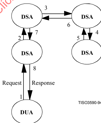
Figure 2 – Uni-chaining mode
