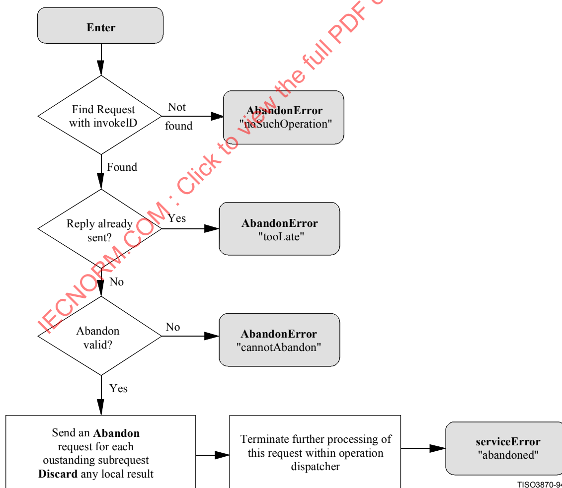
Figure 28 – Abandon procedure
