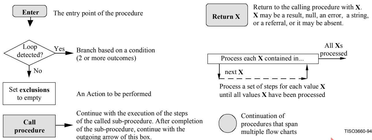
Figure 7 – Symbols Used in Flow Charts
