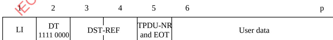
Figure 11 – Data TPDU for class 2
