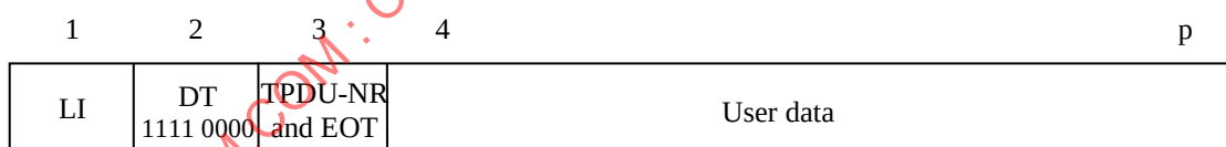
Figure 10 – Data TPDU for class 0
