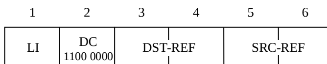
Figure 9 – Disconnect confirm
