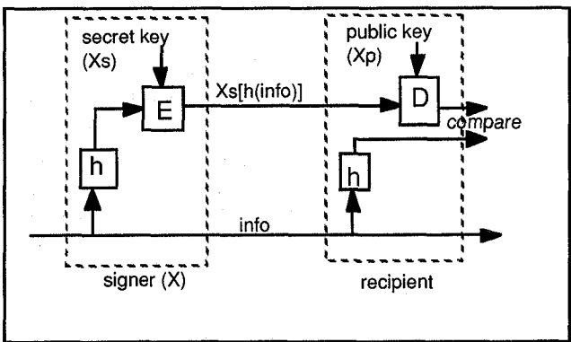
Figure 6 — Digital Signatures
