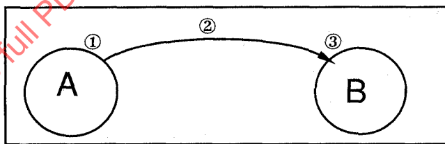
Figure 7 — One-way Authentication
