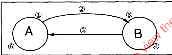
Figure 8 — Two-way Authentication
