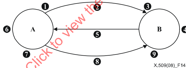
Figure 14 – Three-way authentication
