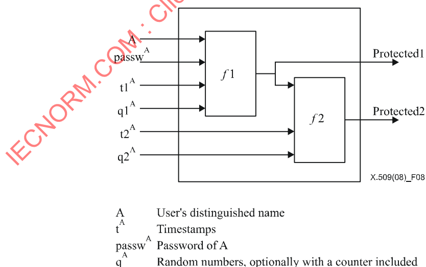
Figure 8 – Protected simple authentication
