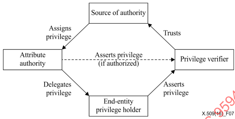
Figure 7 – Delegation model
