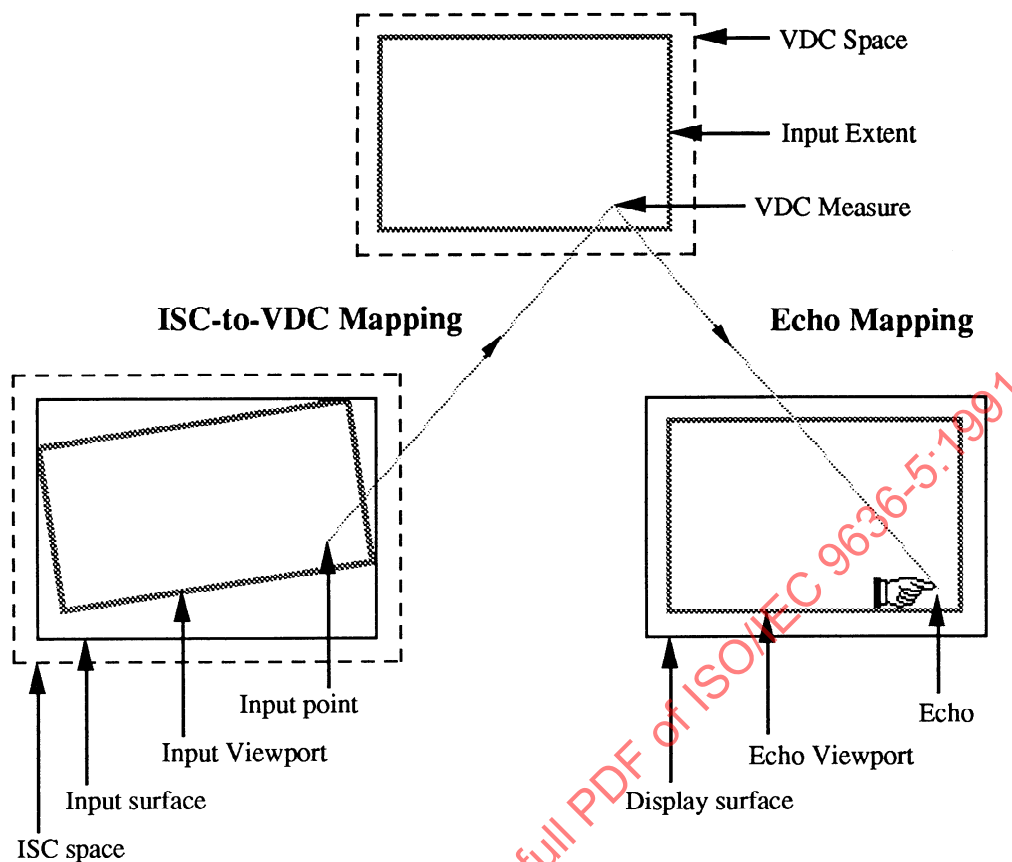
Figure 1 – Input Surface Coordinate mapping
